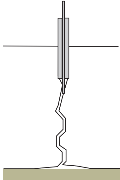
Gang blade cut to re-establish original joint, create deeper center joint to allow for increased penetration to slab base
