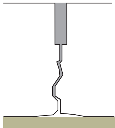
Gravity fill joint with semi-rigid filler- MM-80, MM-80P or Spal-Pro 2000- in multiple passes until filler remains at floor surface level, razor off excess filler above slab flush with floor after cure
